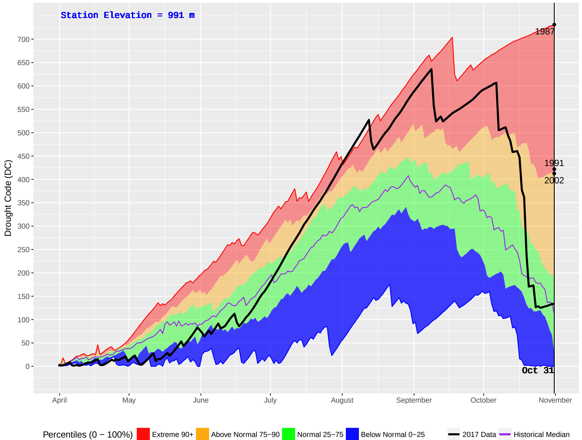
TROUT LAKE (387) : Historical (1987–2016) and Current (2017) Noon Drought Code (DC)
