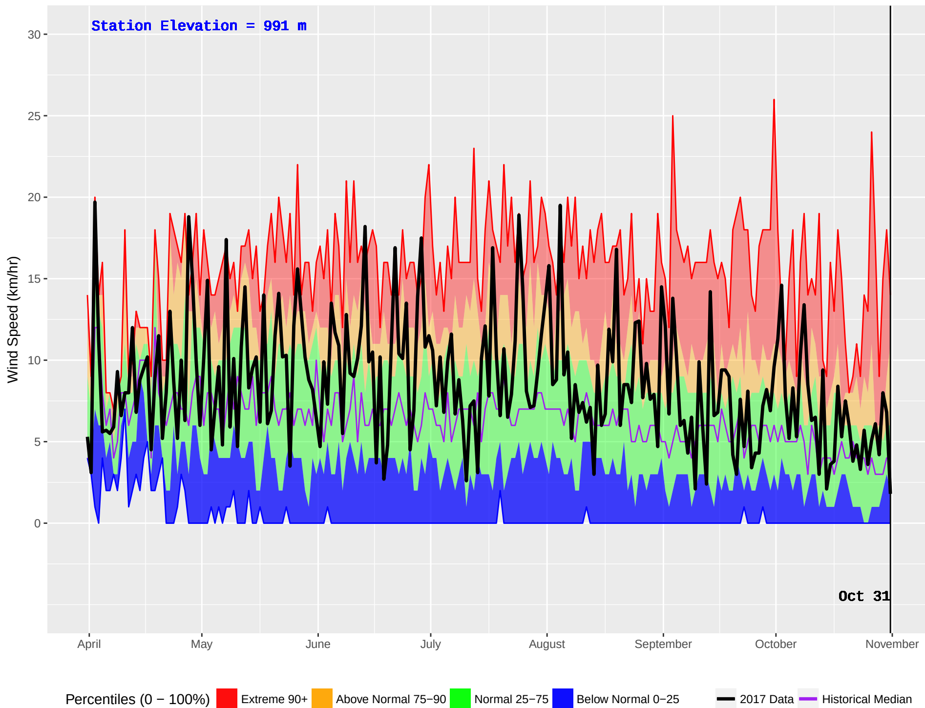
TROUT LAKE (387) : Historical (1987–2016) and Current (2017) Noon Wind Speed
