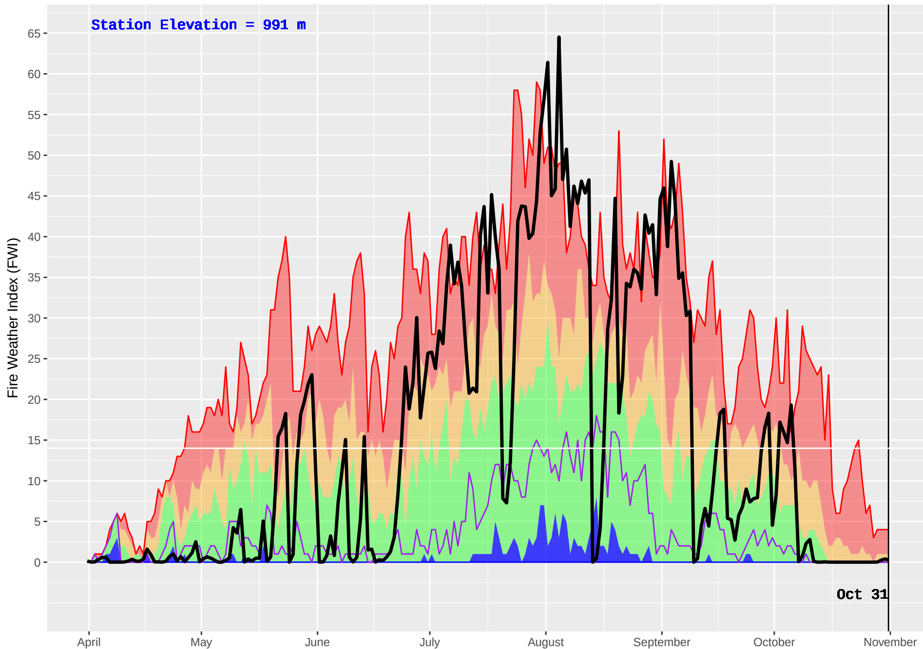
TROUT LAKE (387) : Historical (1987–2016) and Current (2017) Noon Fire Weather Index (FWI)
